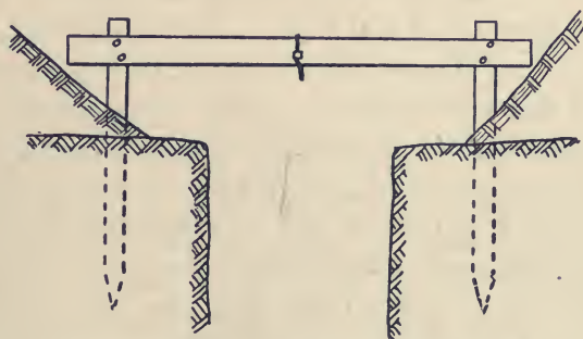
FIG. 6.—METHOD OF SETTING GRADE-PLANK.
